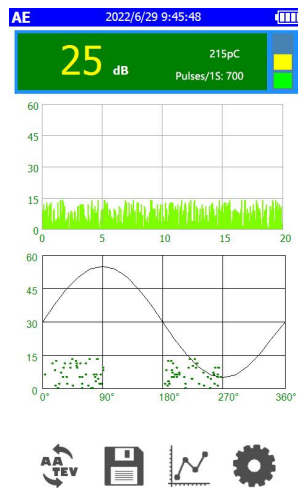
Time-domain signal waveforms and PRPD phase maps
