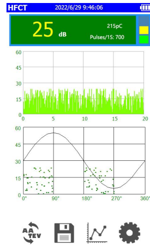
HFCT test interface
