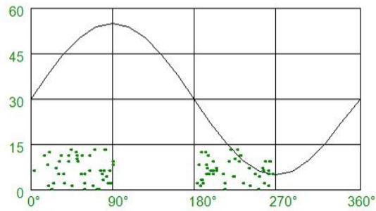
PRPD atlas
