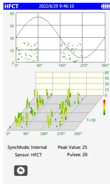
PRPD and PRPS atlas
